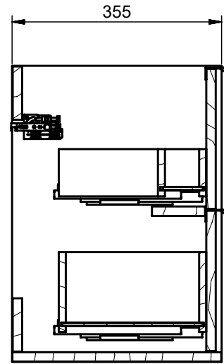
B-B (1:7)
